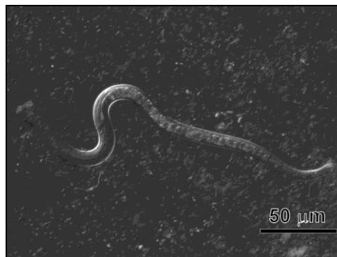
Figure 1. Nematode in the gut content of proteus from Stobe cave (photo: R. Kostanjšek).
